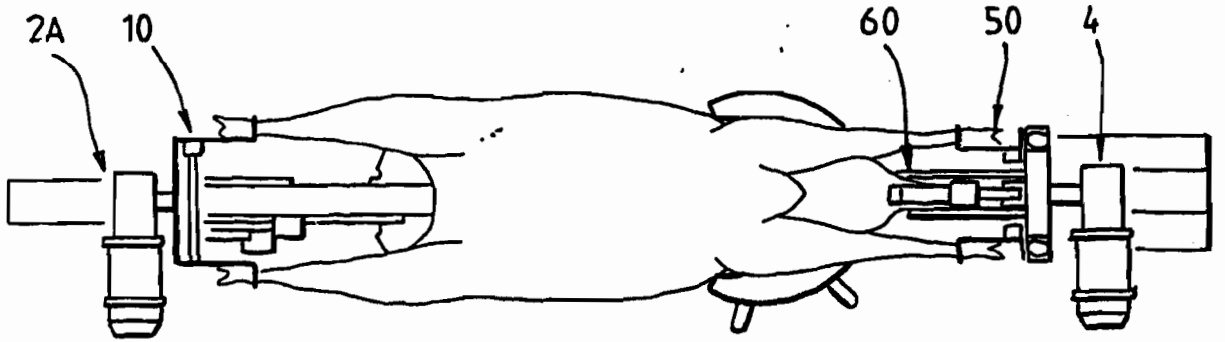
FIG. 14. Shearing position 1
