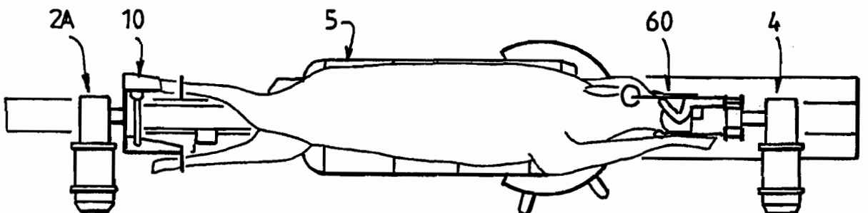
FIG. 19. Shearing position 6
