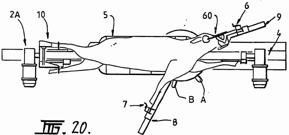
Shearing position 7
