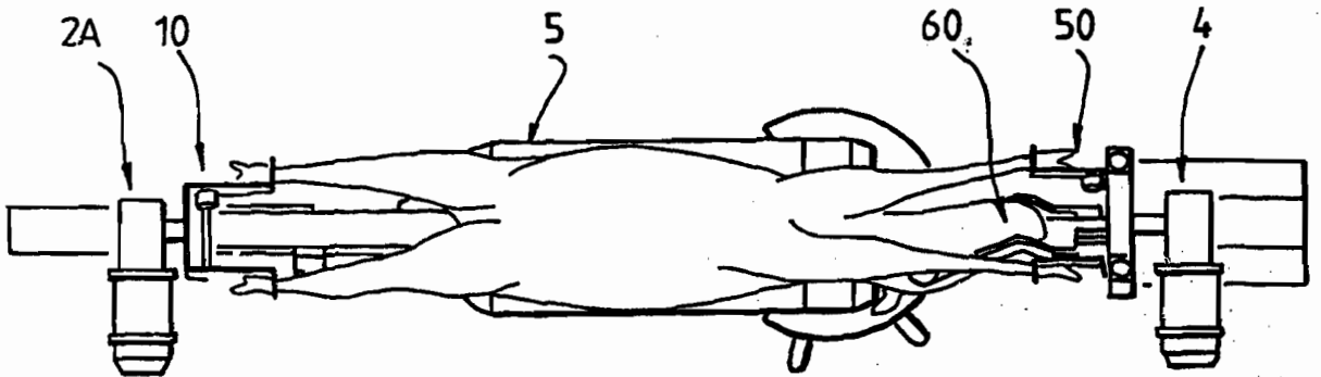
FIG. 15. Shearing position 2
